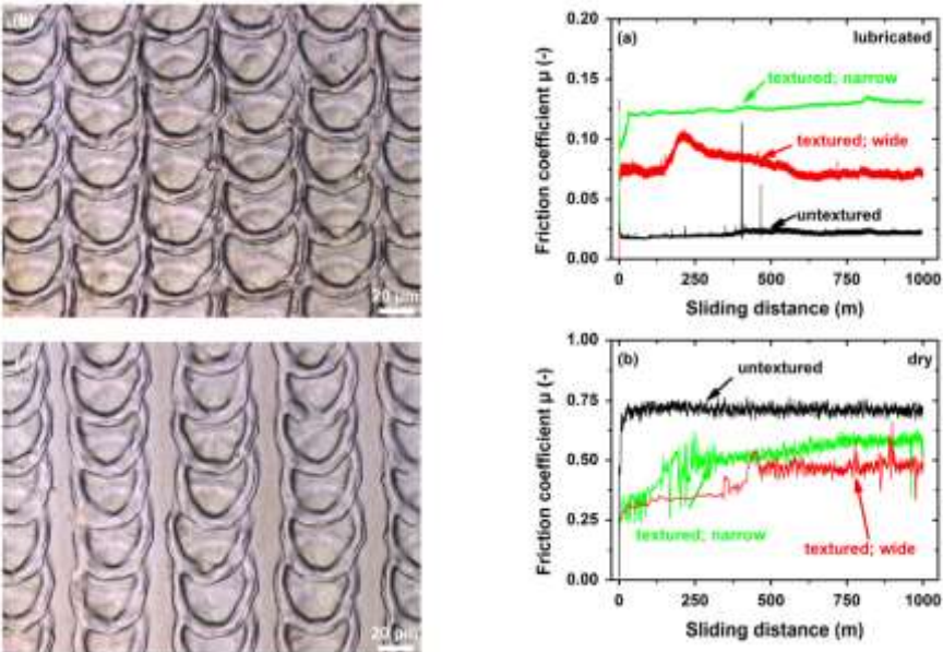
Images of bio-inspired surface morphologies created through laser surface texturing (left) and their effect on friction coefficient in lubricated and dry condition (right) from [2].
