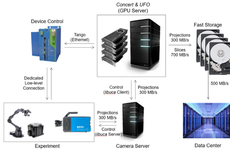
Figure 1: KARA's data acquisition system
